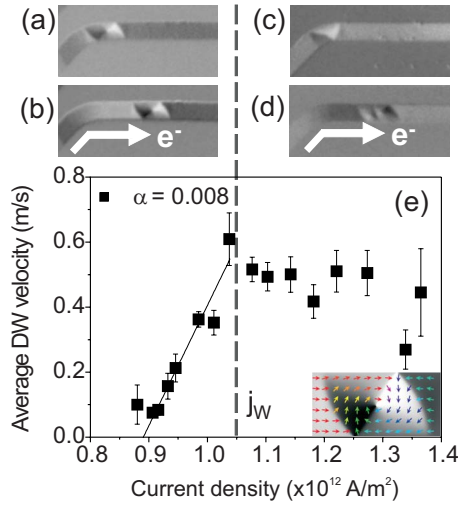
FIG. 1. (Color online) XMCD-PEEM images taken [(a) and (c)] before and [(b) and (d)] after a current pulse of duration 25 \mu\text{s} and density j \sim 10^{12} \text{ A/m}^2 . For j < 1.05 \times 10^{12} \text{ A/m}^2 , the DW motion occurs without spin-structure transformations. For j > 1.05 \times 10^{12} \text{ A/m}^2 , vortex-core nucleation and annihilation, and propagation of multivortex walls occurs. (e) Average DW velocity v as a function of current density j determined by XMCD-PEEM imaging, for 1500-nm-wide, 20-nm-thick Py wires. Below the Walker threshold current density j_w the data are fitted by Eq. (2). The inset is a simulation of a vortex wall in a Py wire with contrast equivalent to the XMCD-PEEM images (a) and (b).
